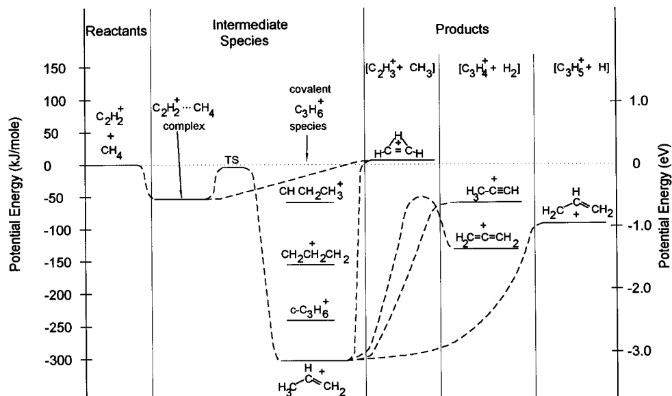
FIGURE 2. Reaction coordinate diagram for the C_3H_6^+ system, showing reactants, products, and intermediates.
